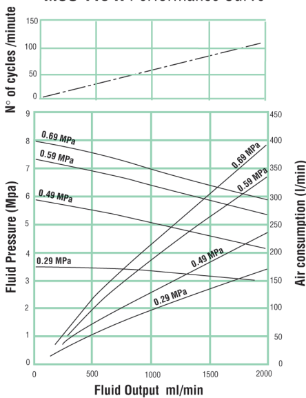
MSU 113 N Performance Curve
