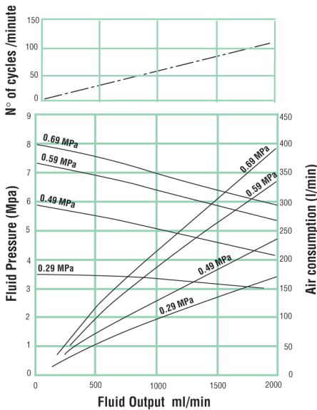
MSU 113 N Performance Curve
