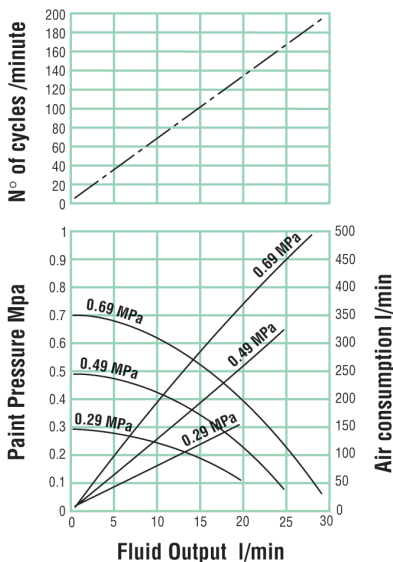
DPS 120-B Performance Curve
